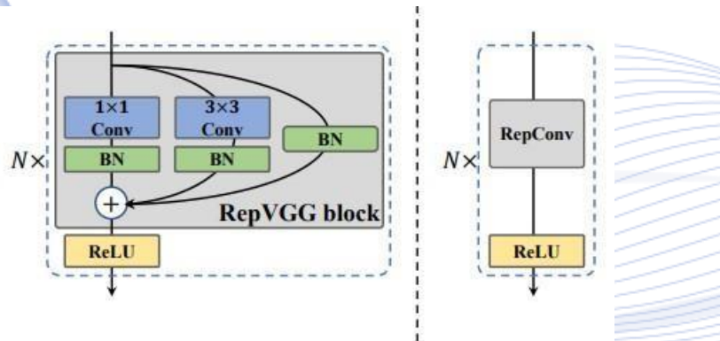
RepVGG [DING2021] building block.
